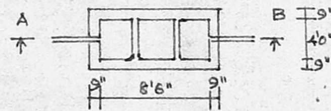
DETAILS OF SEPTIC TANK
