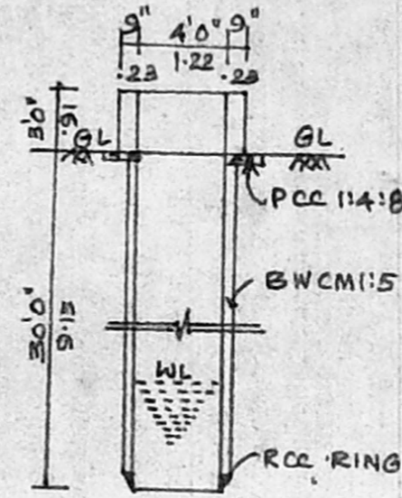
WELL DETAILS
