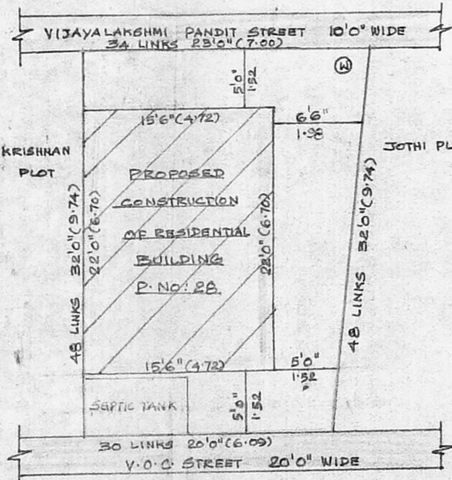
SITE PLAN
